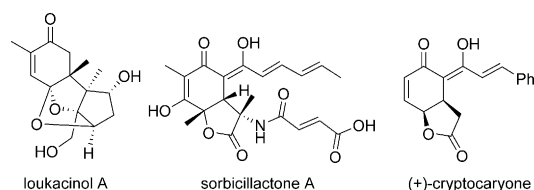
Figure 1. Examples of tetrahydrobenzofuranones isolated from natural sources.
